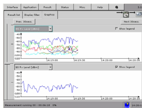
Figure 2 Graphical presentation of GSM Abis interface MEASUREMENT_RESULT message information.
